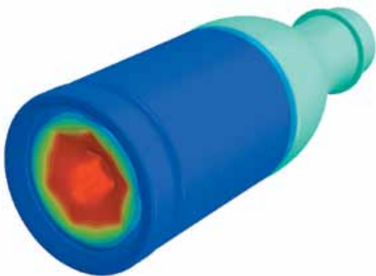
A side view of an Abaqus FEA analysis of a vacuum deformation shows that the greatest load (red) occurs at the bottom of the container.
